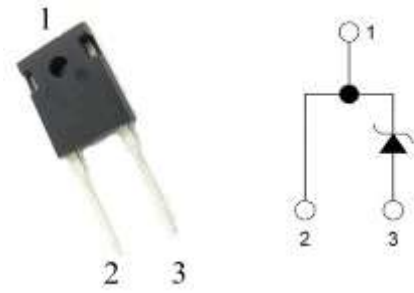
TO-247-2
