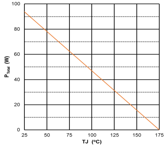
Figure 4. Power Derating
